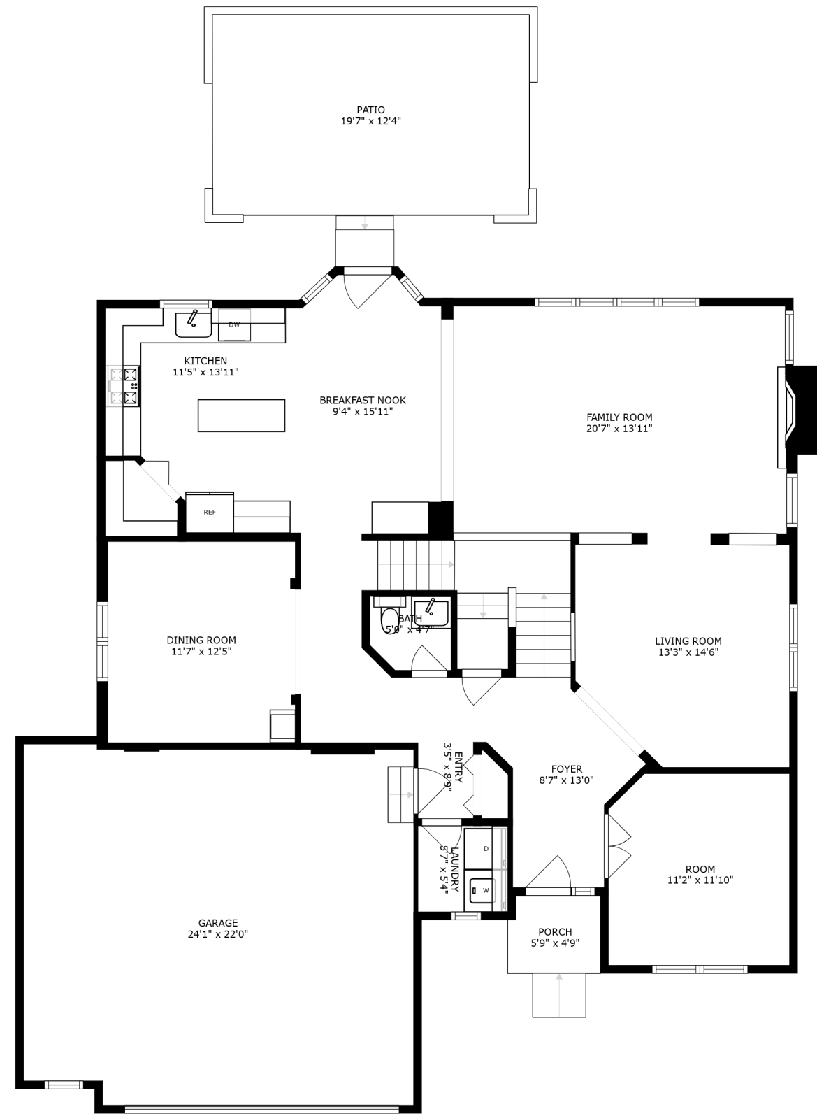
FLOOR 2
