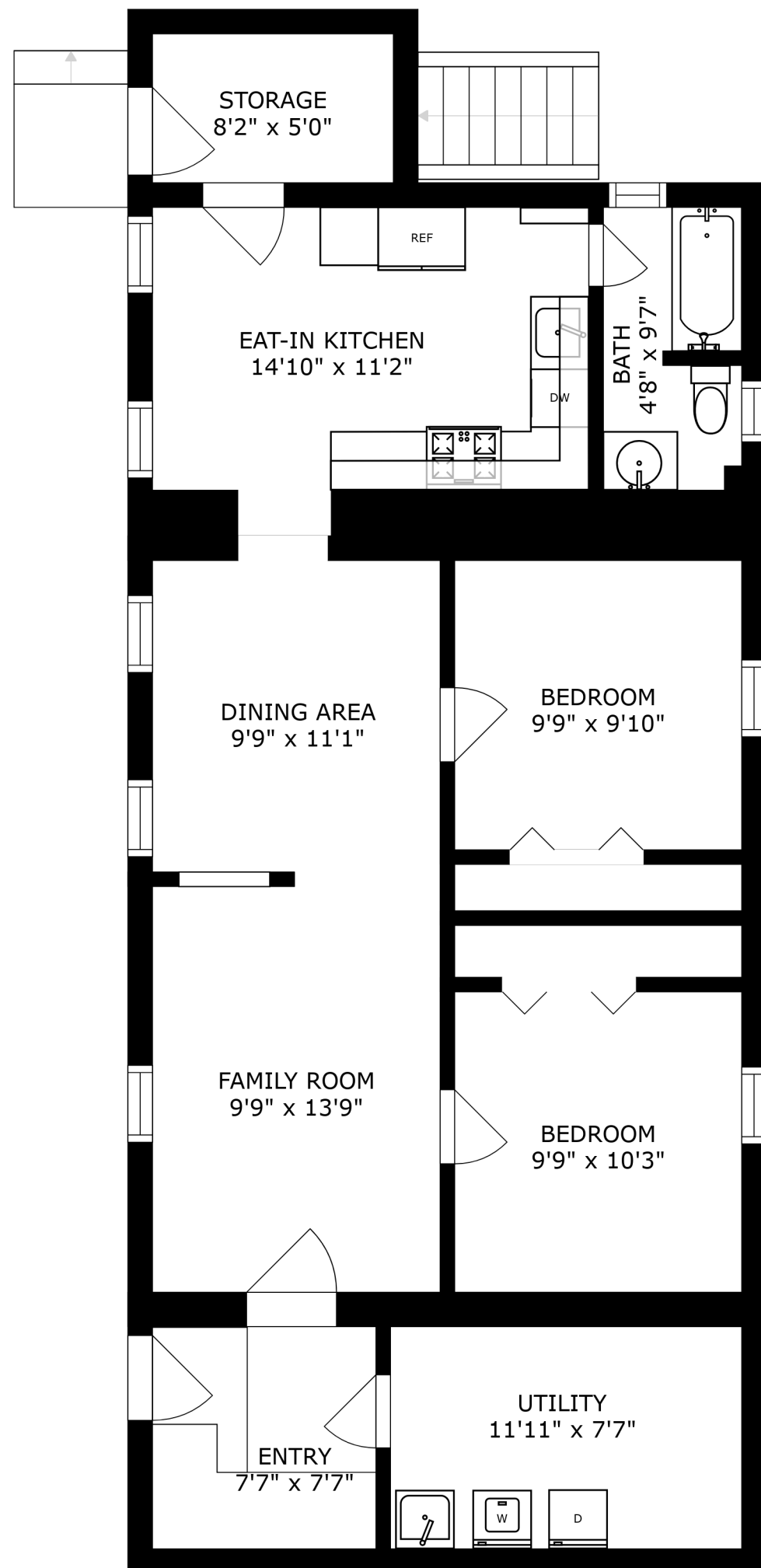
FLOOR 1
