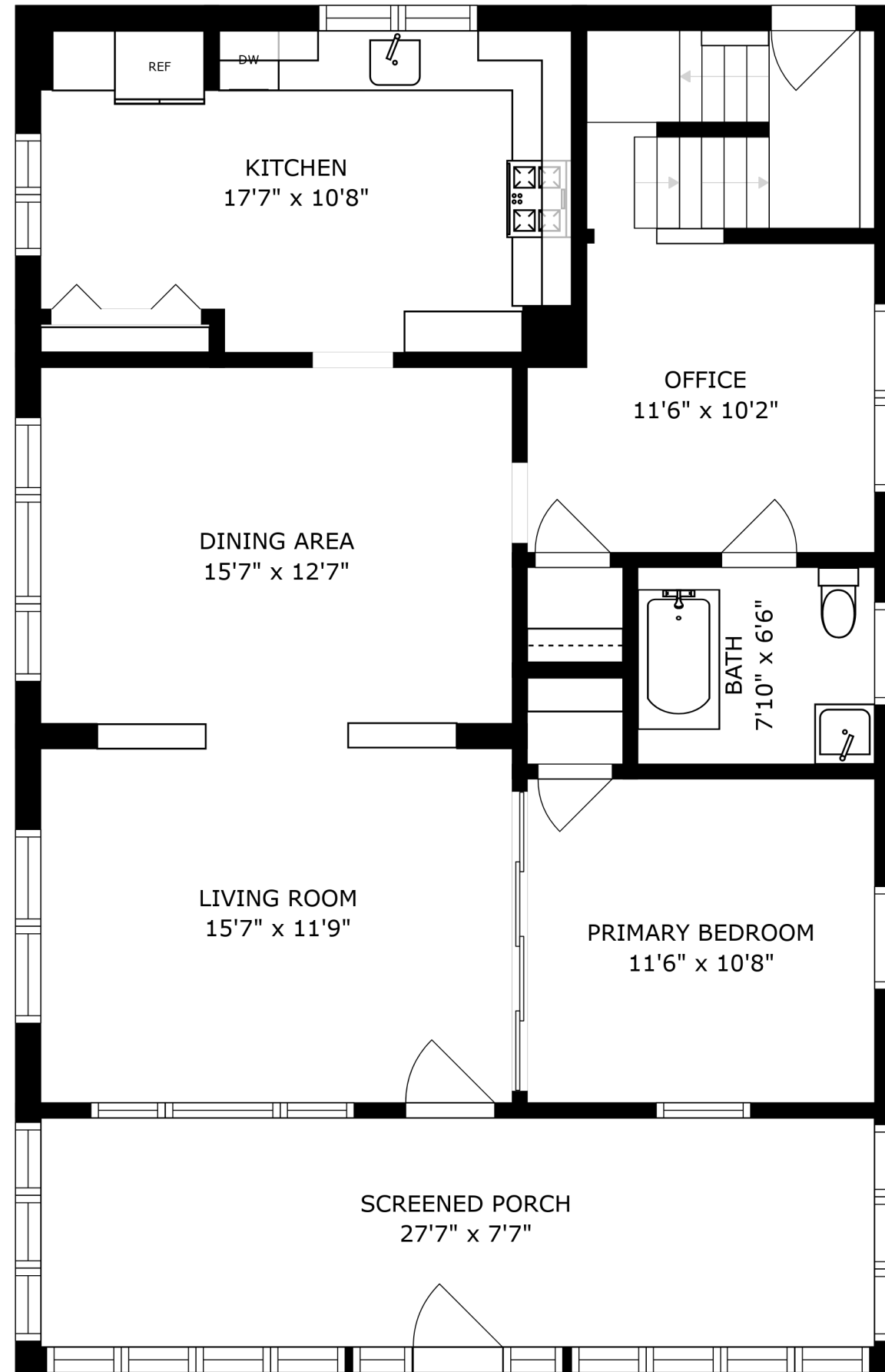
FLOOR 2
