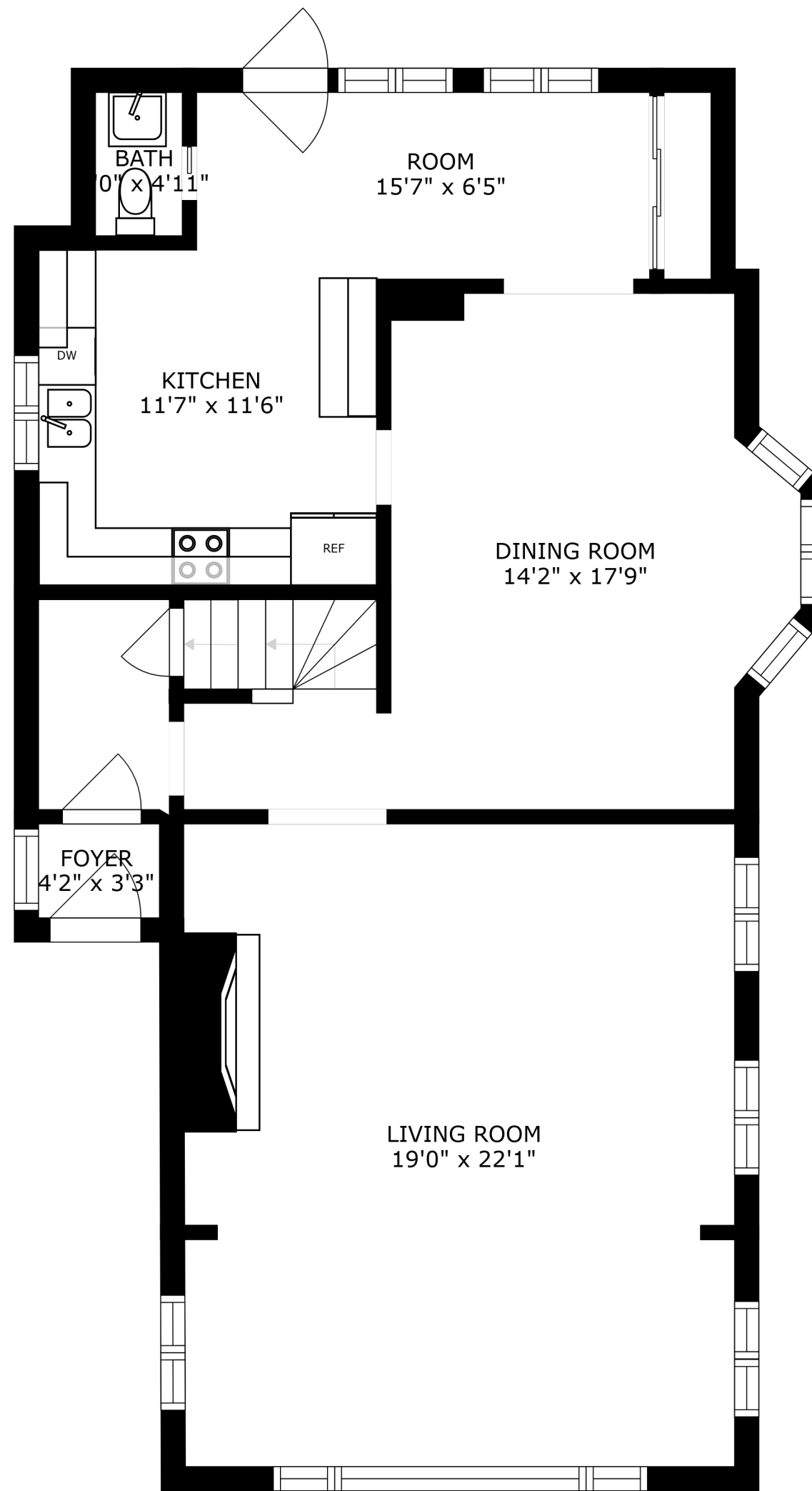
FLOOR 2
