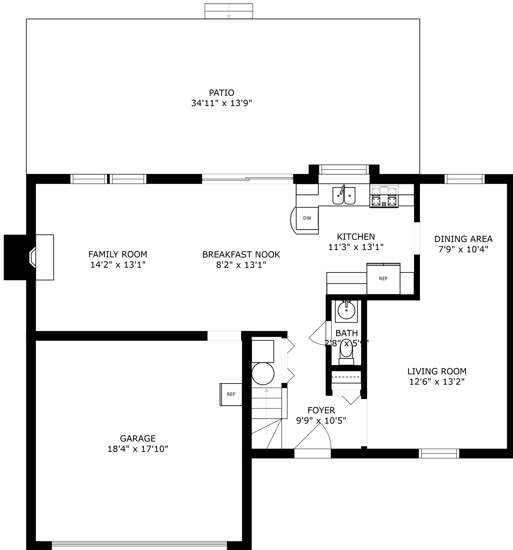
FLOOR 1
