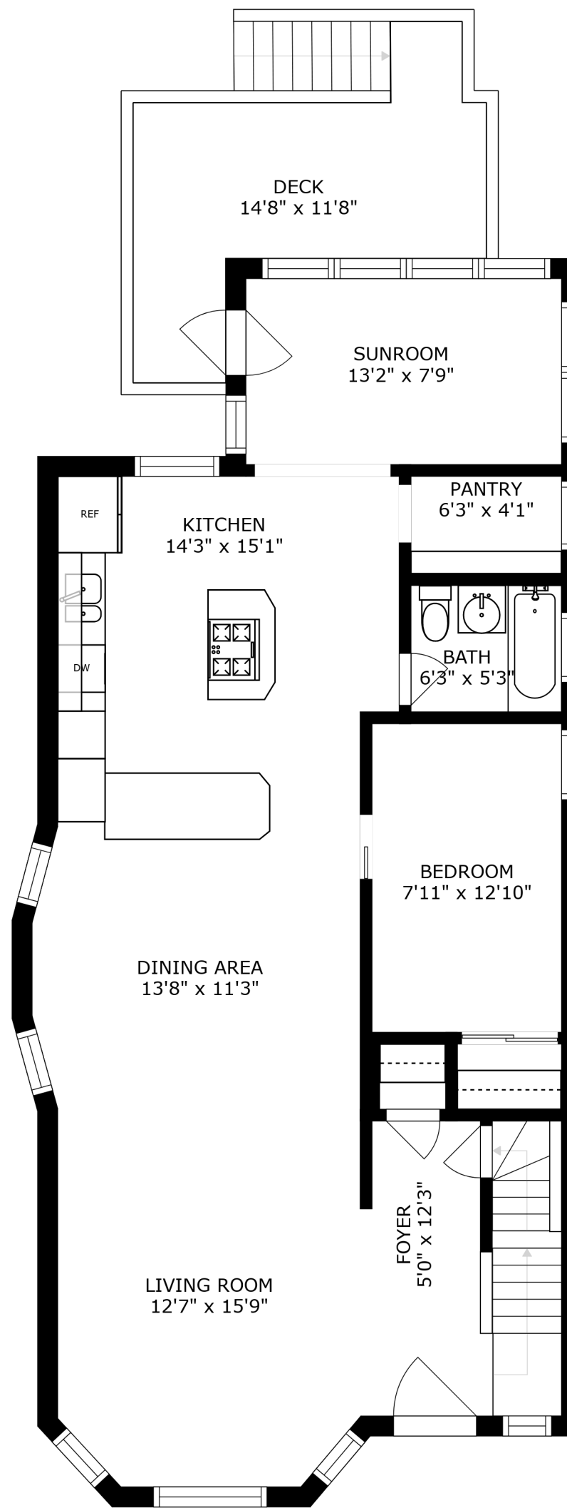
FLOOR 2
