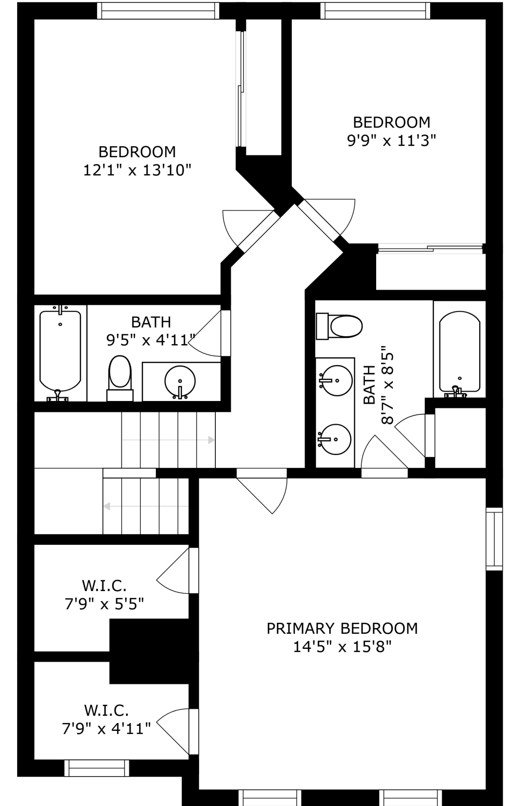
UPPER LEVEL
