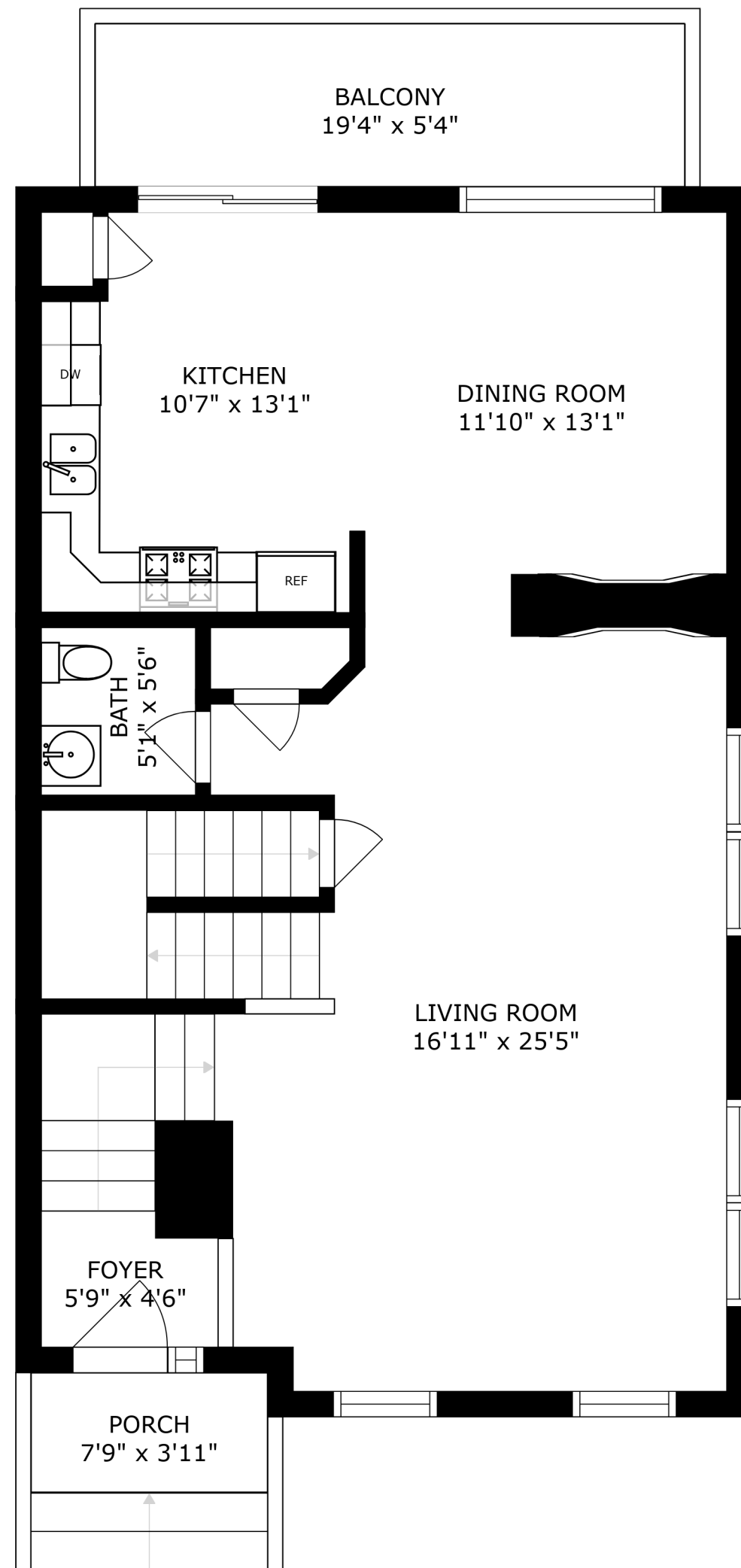
MAIN LEVEL
