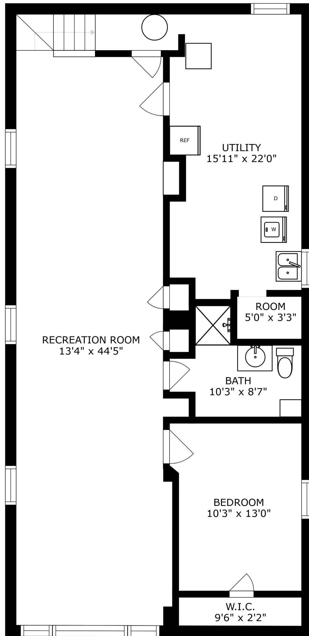
FLOOR 1
