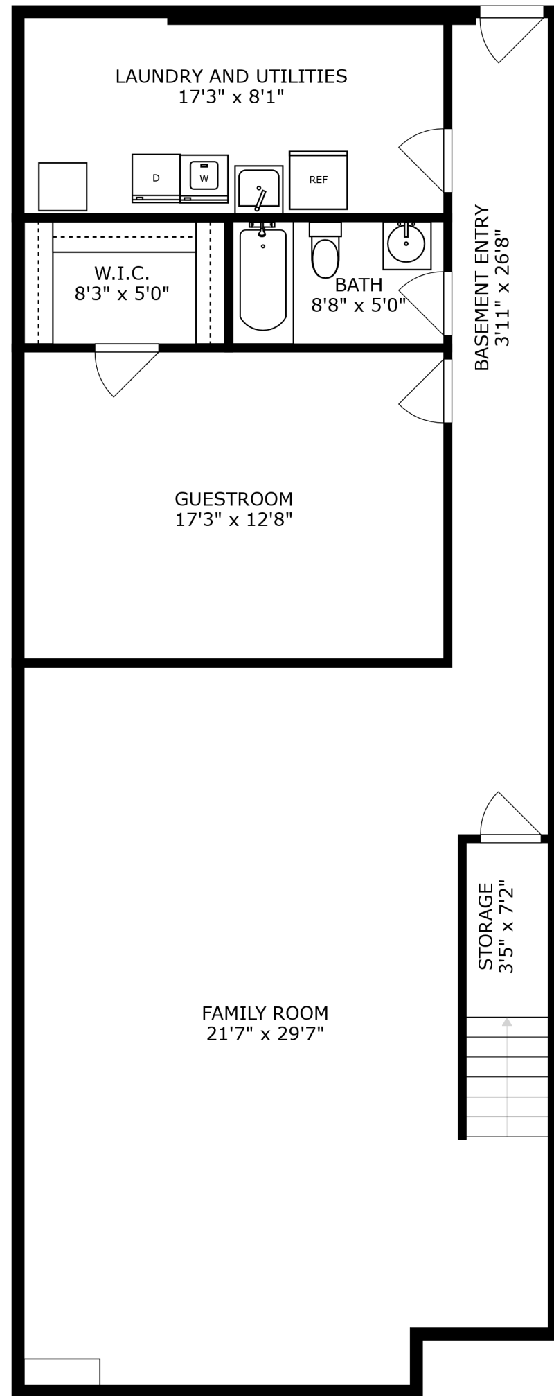
FLOOR 1
