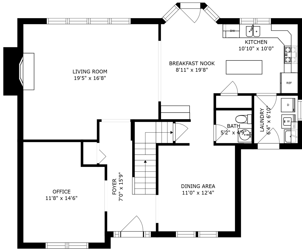
FLOOR 2
