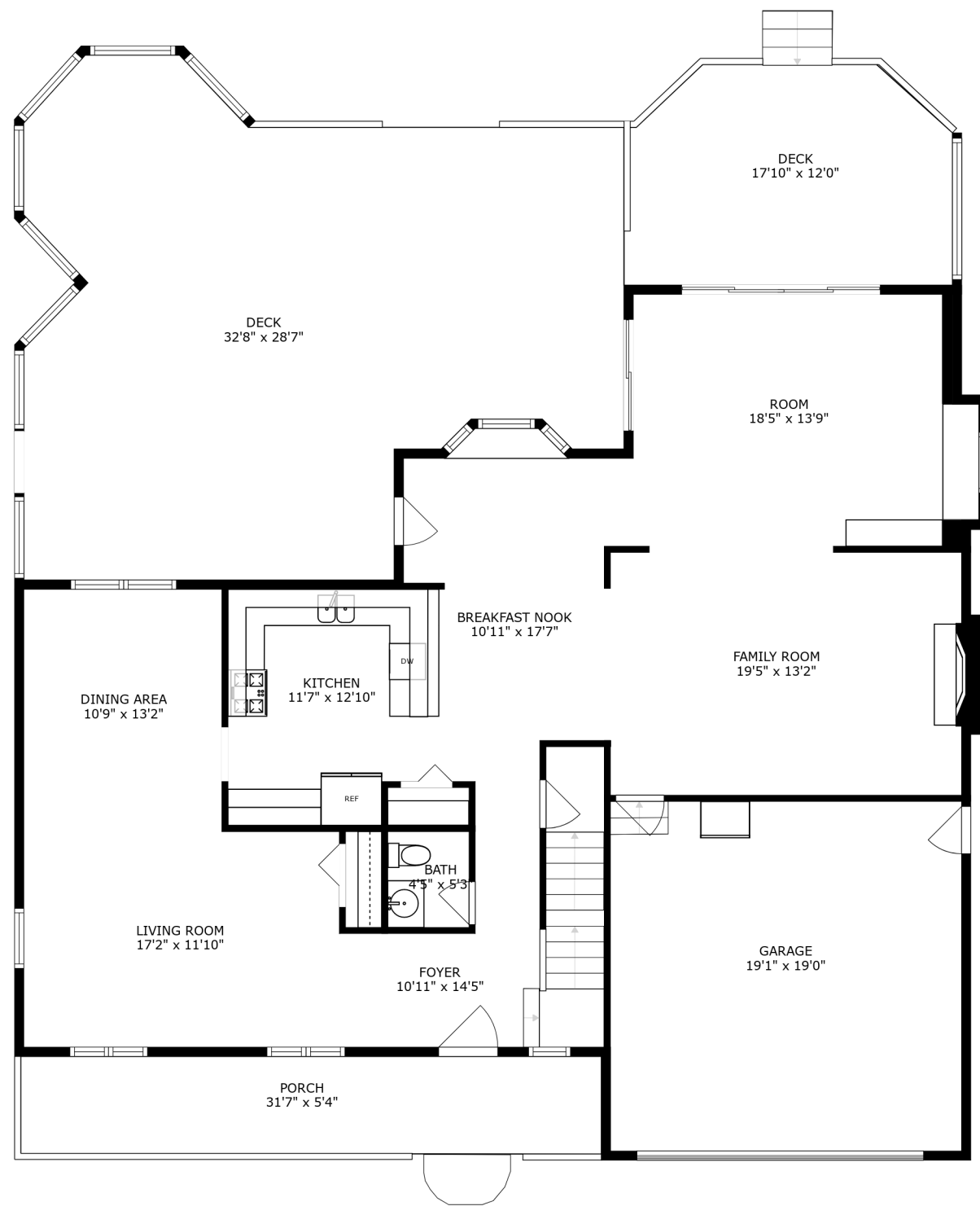
FLOOR 2
