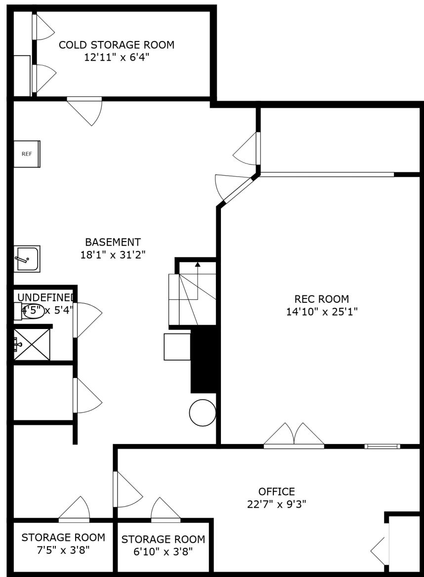
FLOOR 1
