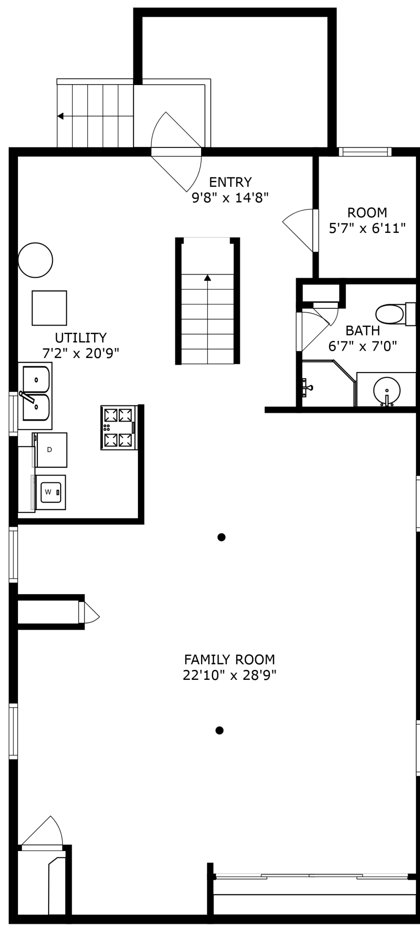
FLOOR 1
