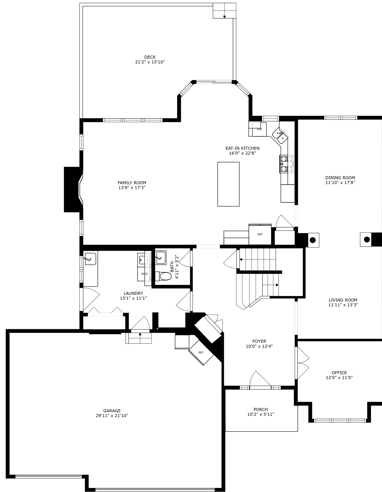
FLOOR 2
