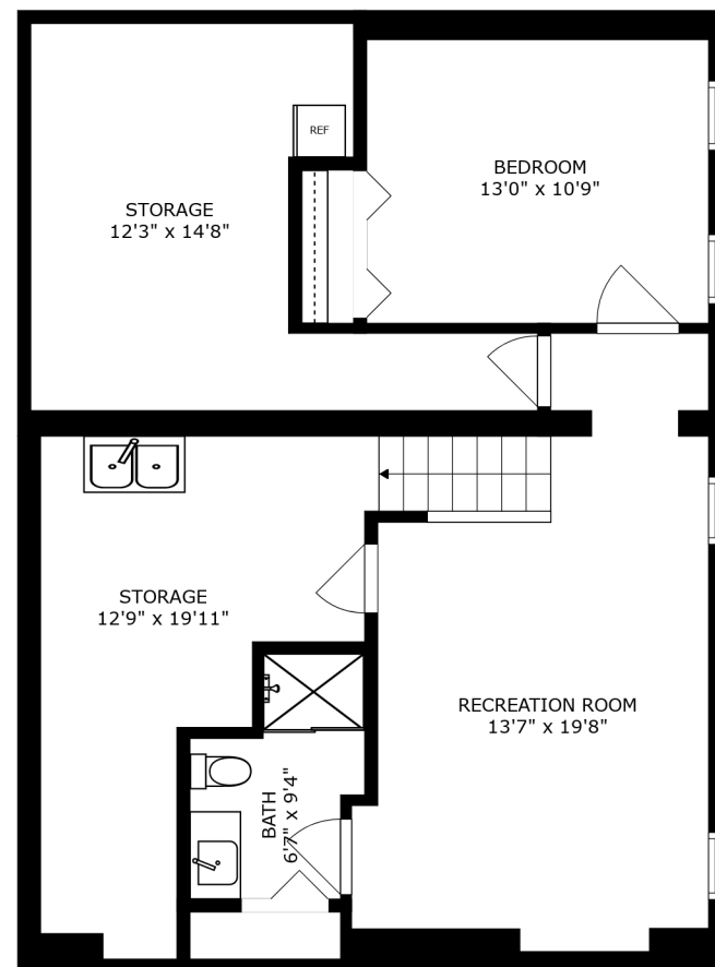
FLOOR 1
