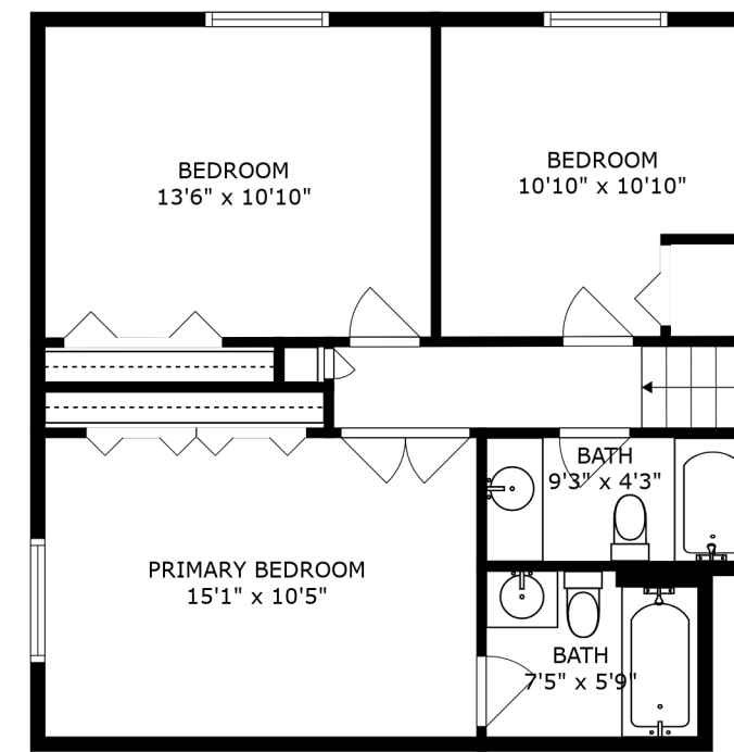
FLOOR 3
