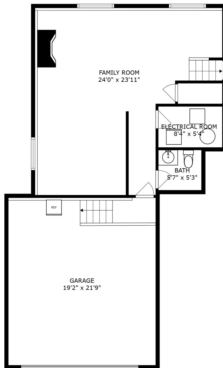
FLOOR 1
