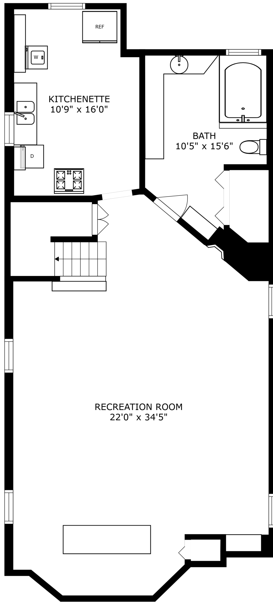
FLOOR 1
