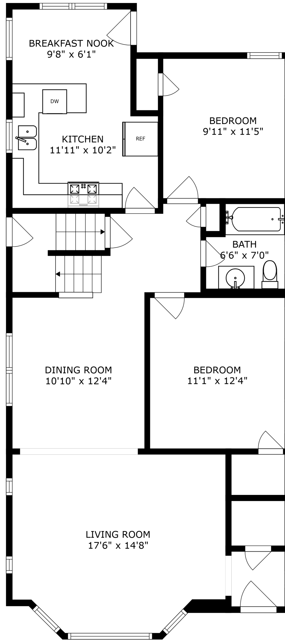
FLOOR 2
