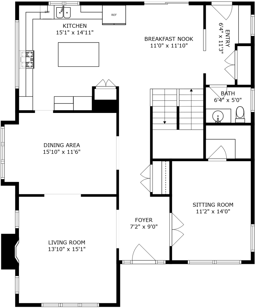
FLOOR 2
