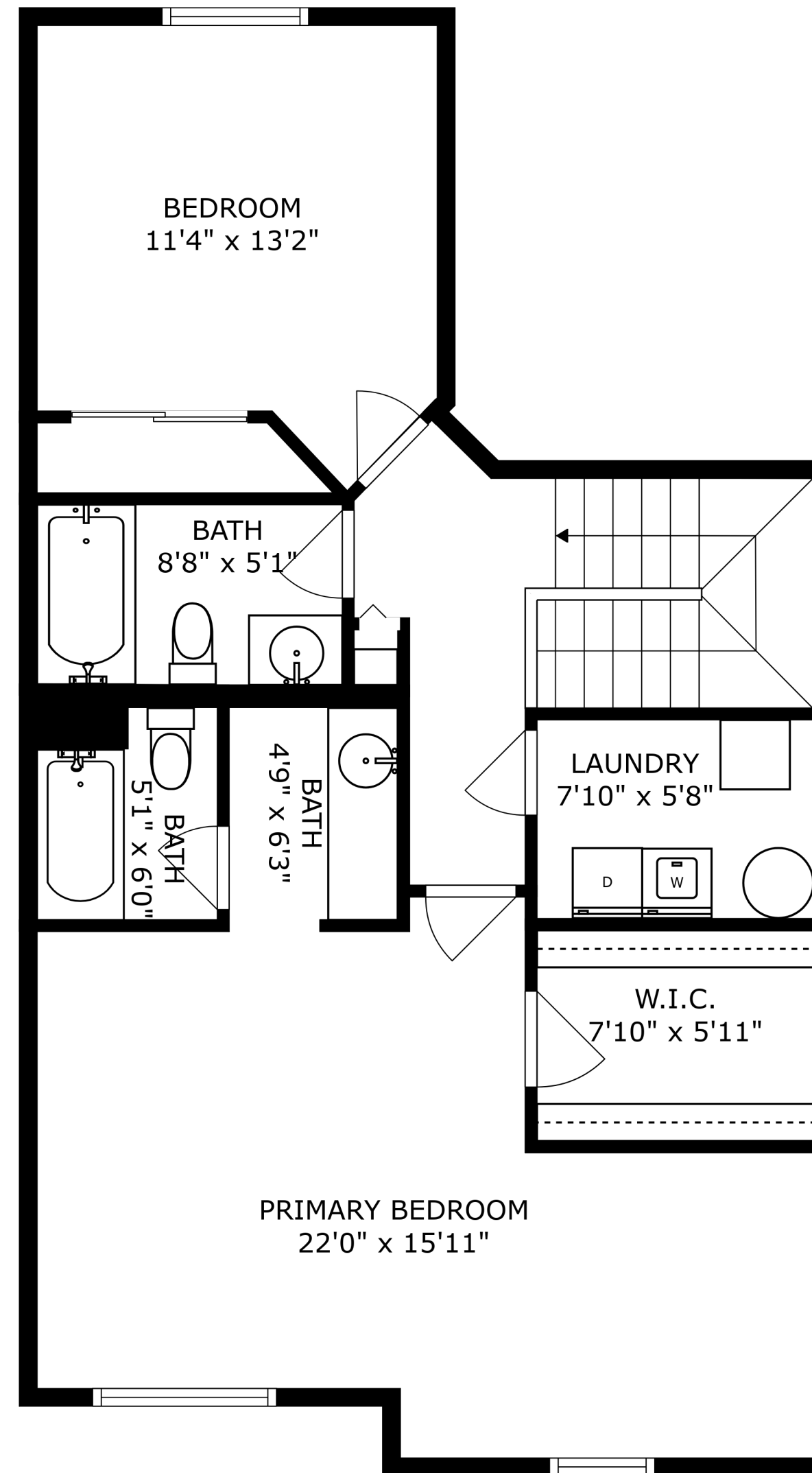
FLOOR 2
