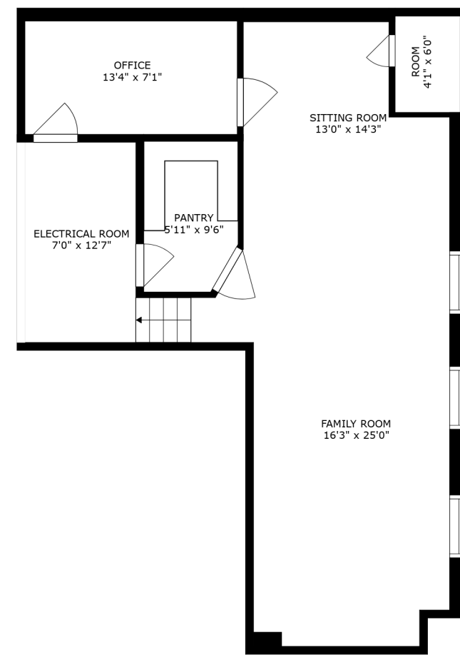
FLOOR 1
