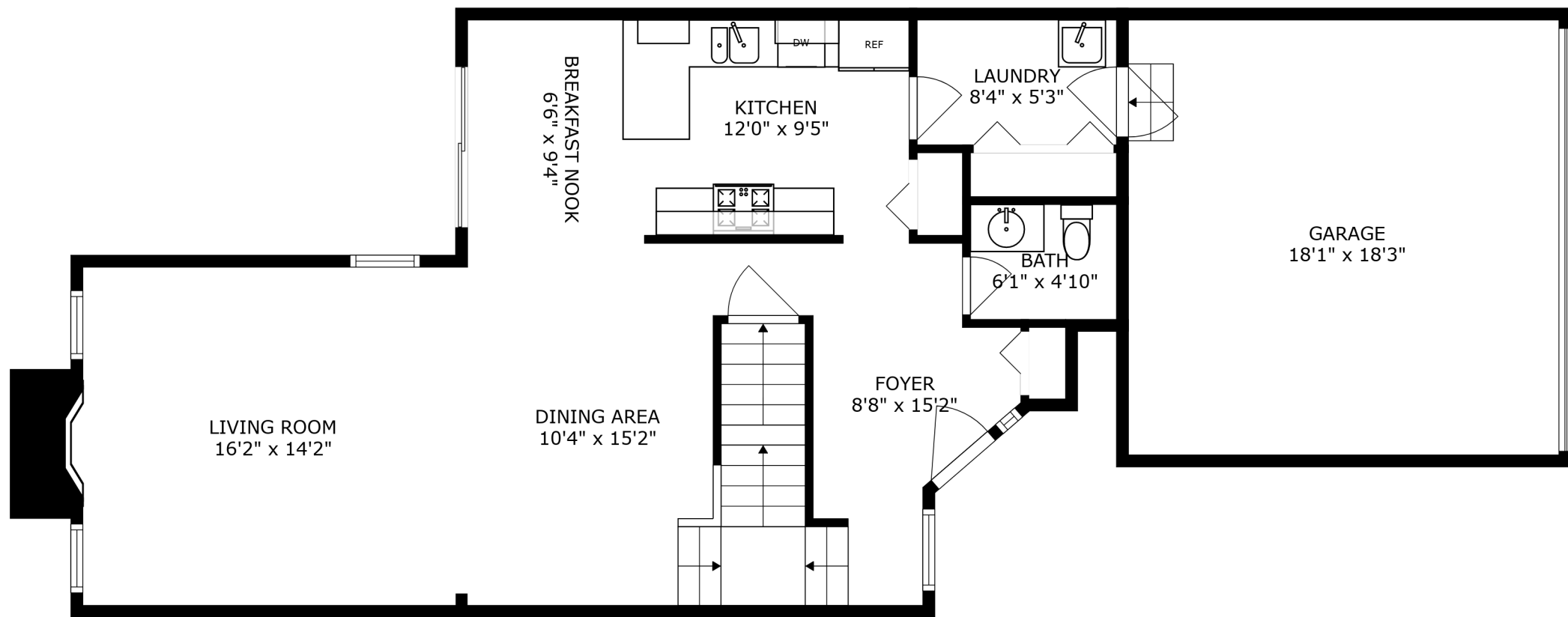
FLOOR 2
