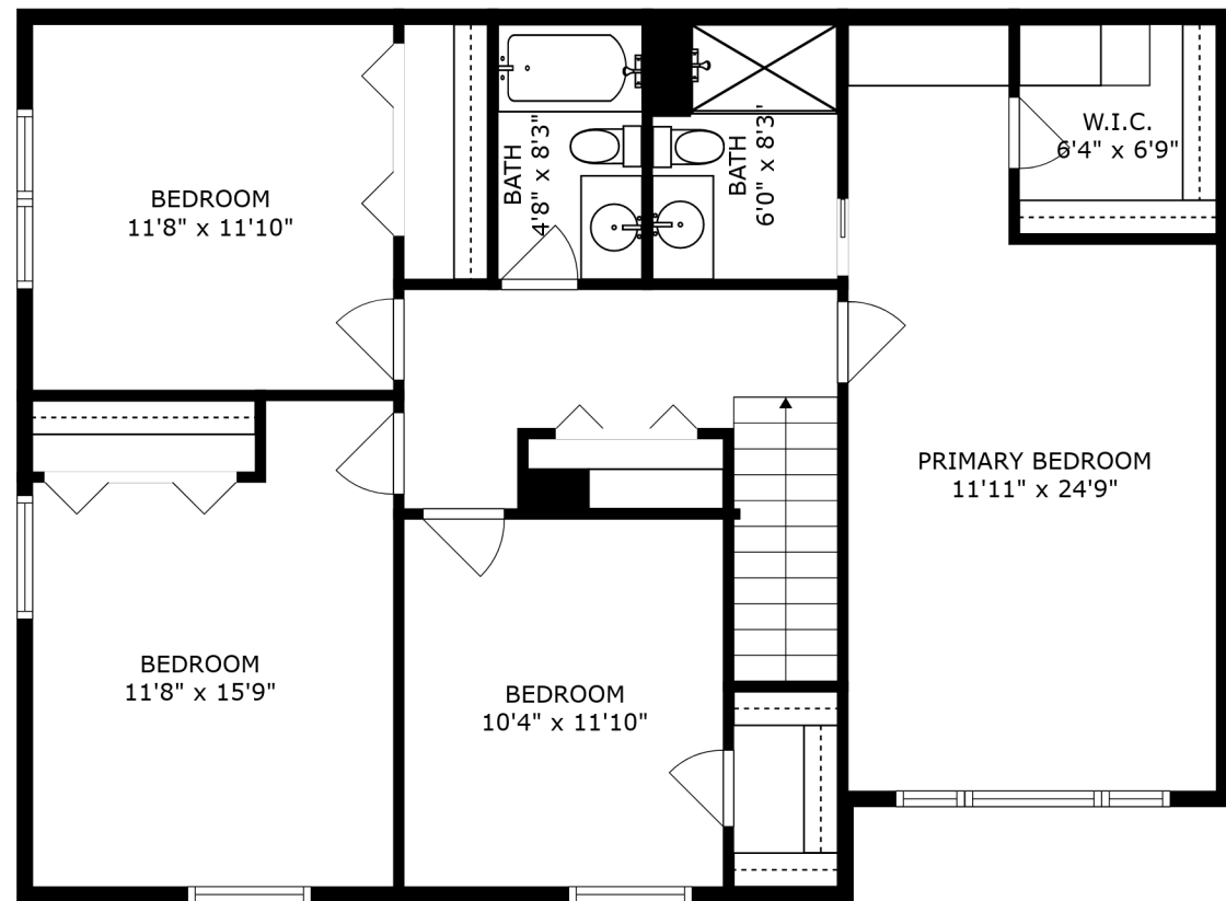
FLOOR 3
