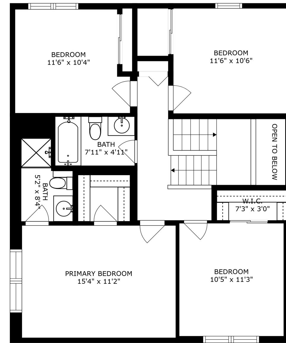
FLOOR 3
