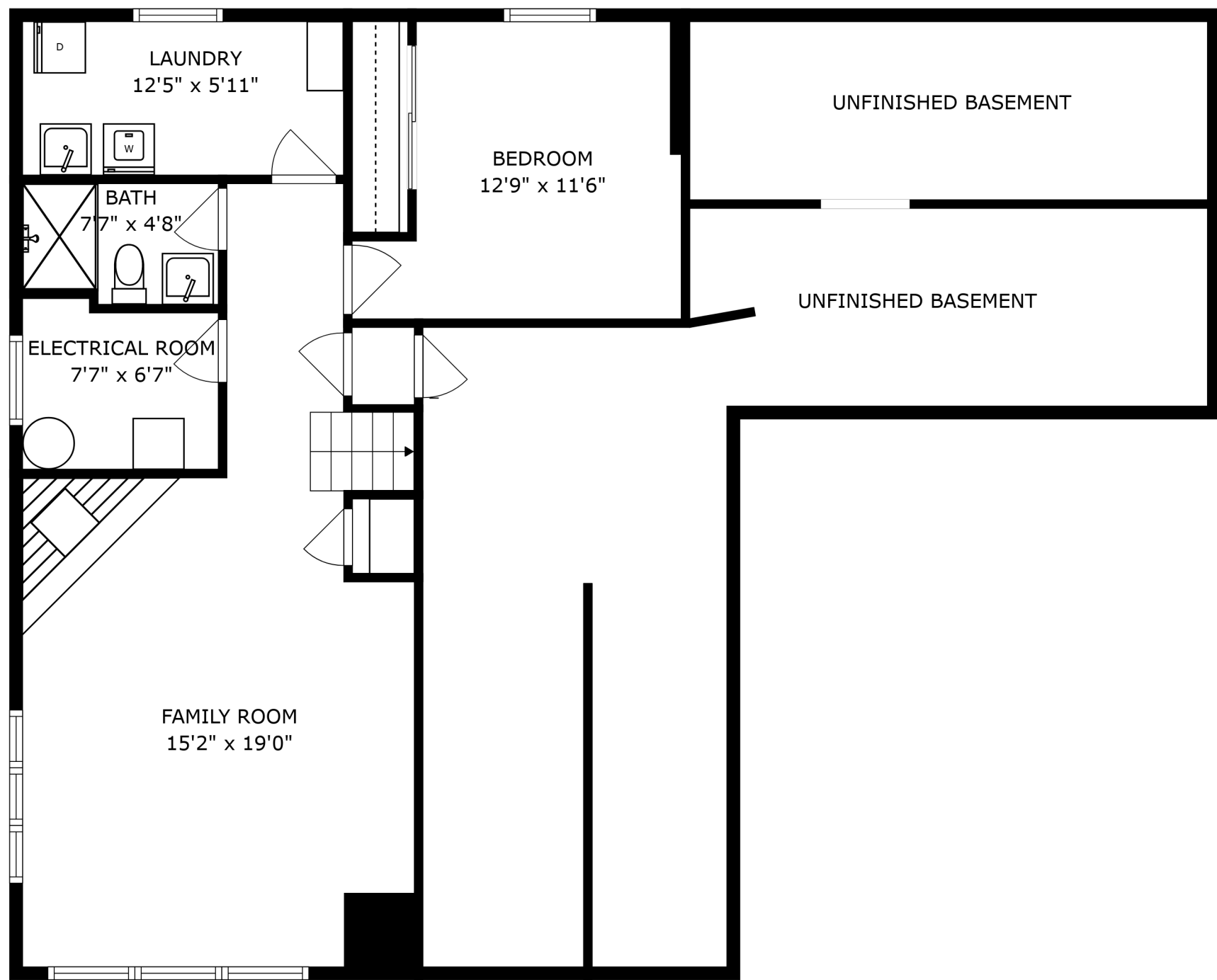
FLOOR 1
