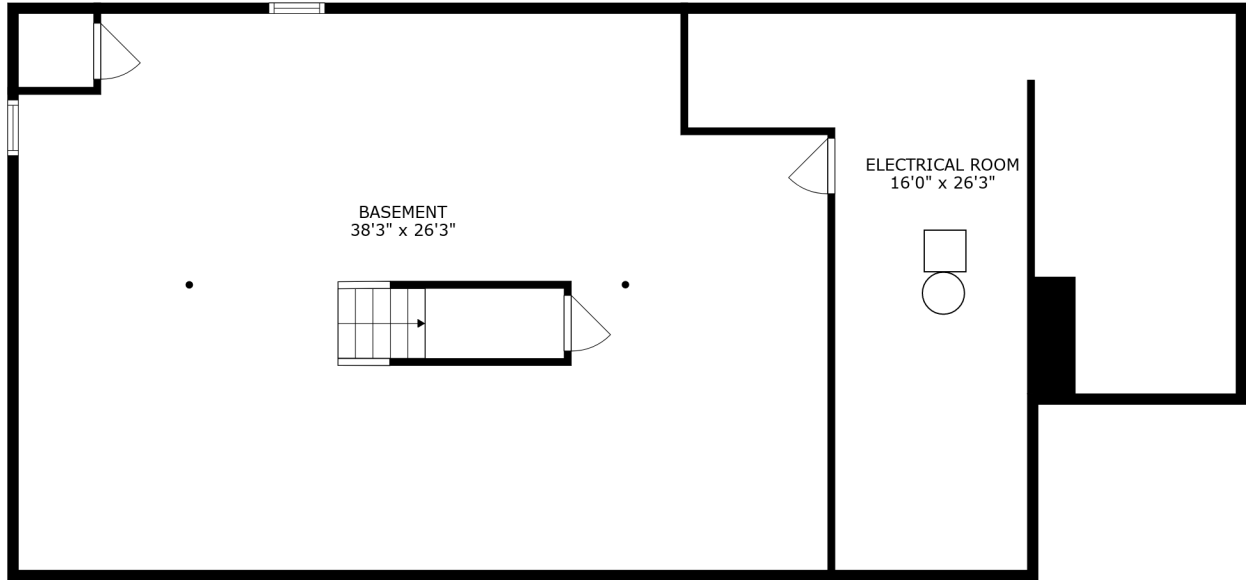
FLOOR 1
