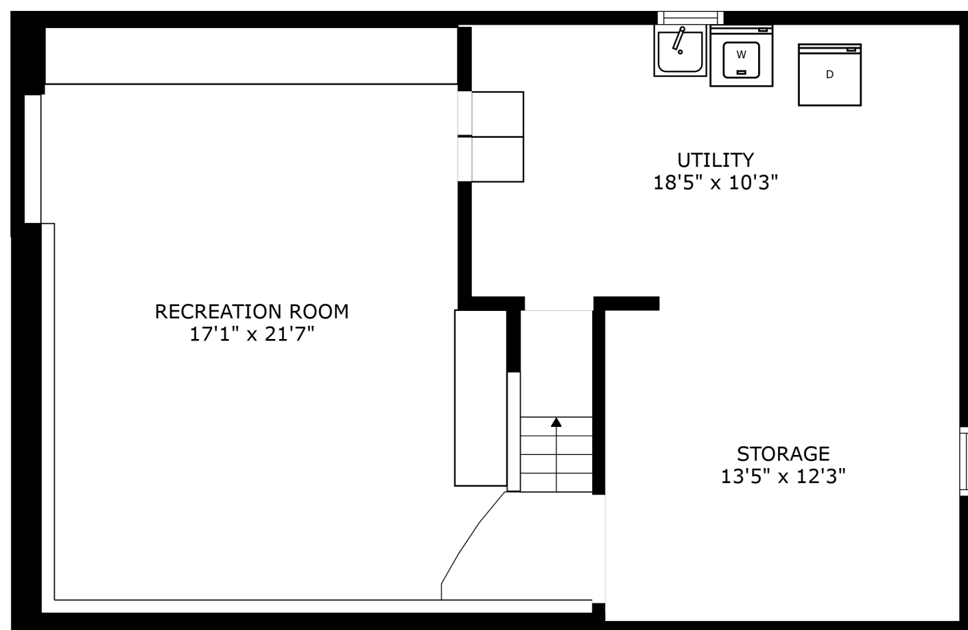
FLOOR 1
