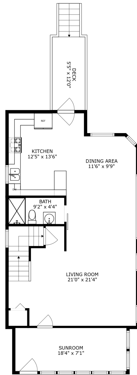
FLOOR 2
