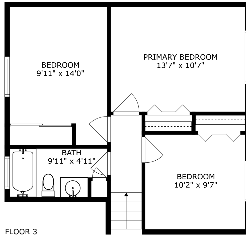
FLOOR 3
