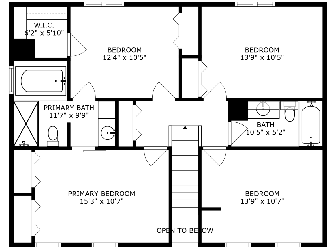
FLOOR 3
