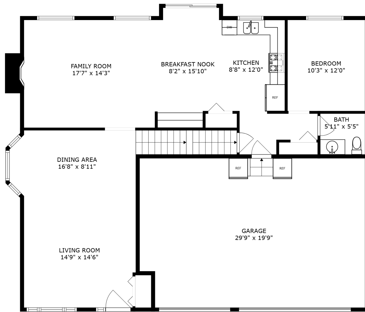
FLOOR 2
