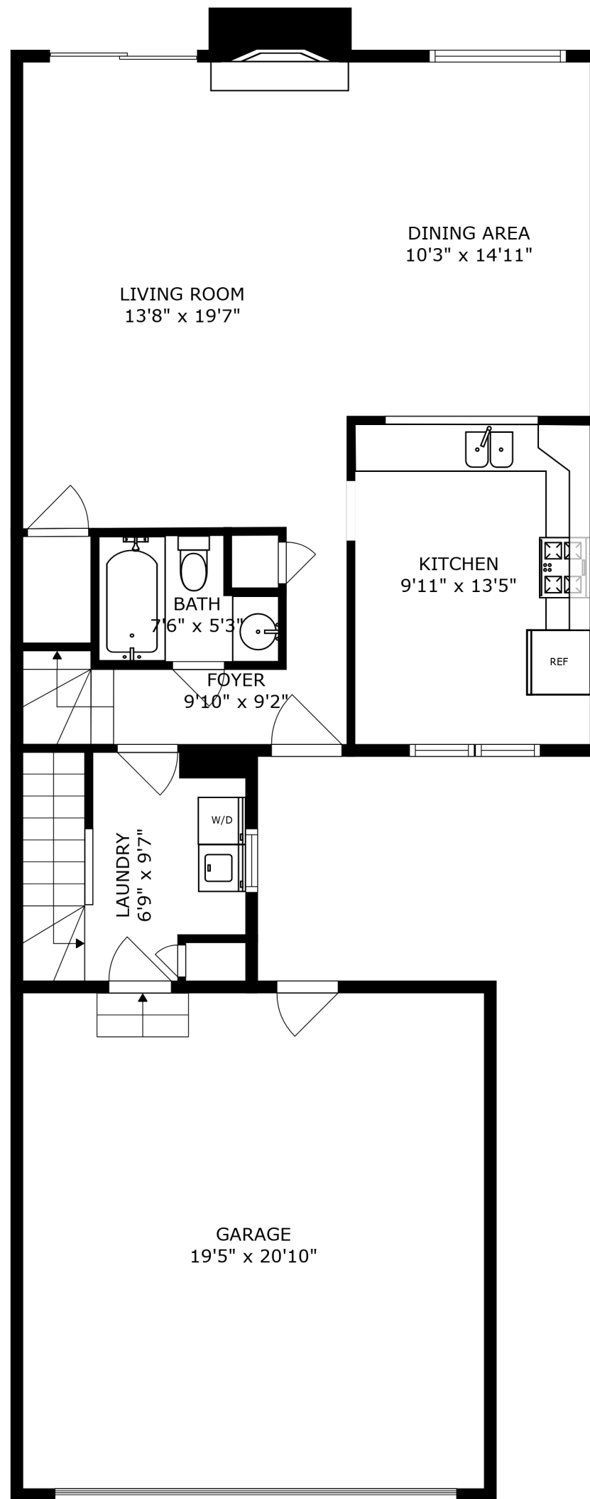
FLOOR 2
