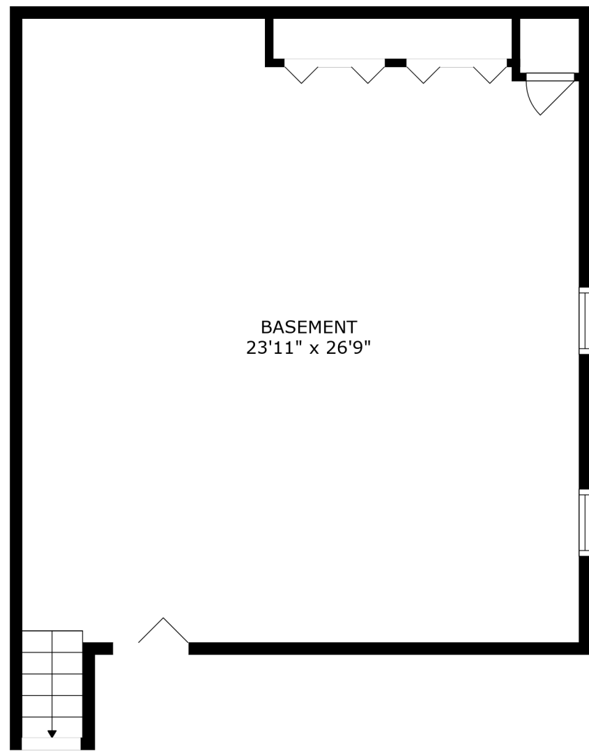
FLOOR 1
