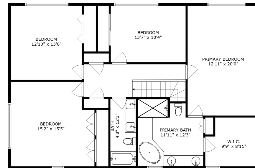
FLOOR 3
