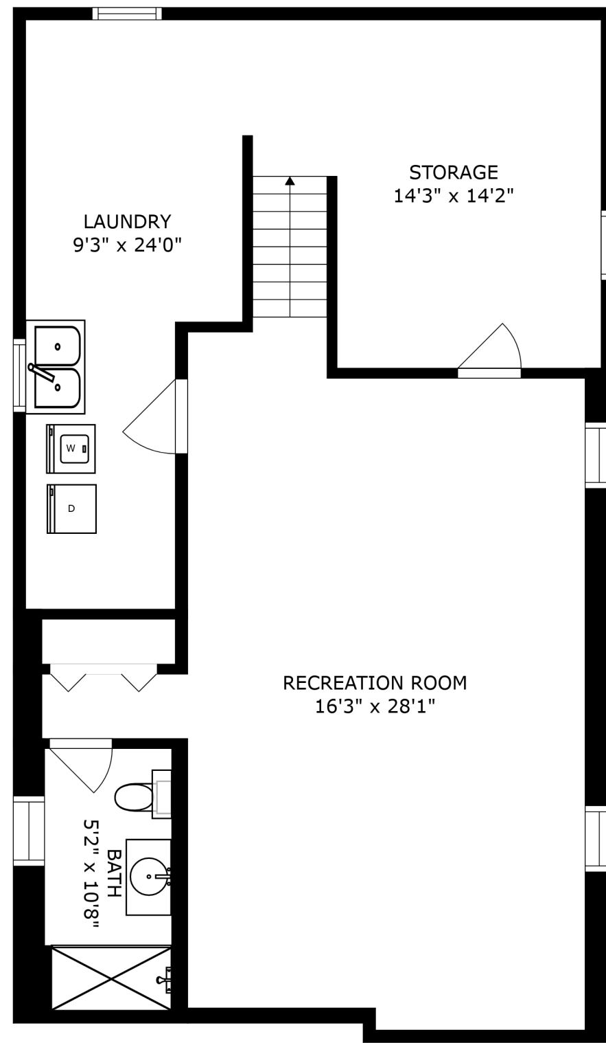
FLOOR 1
