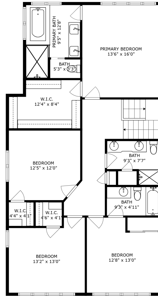
FLOOR 4
