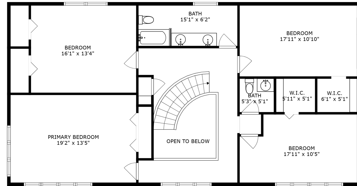
FLOOR 3
