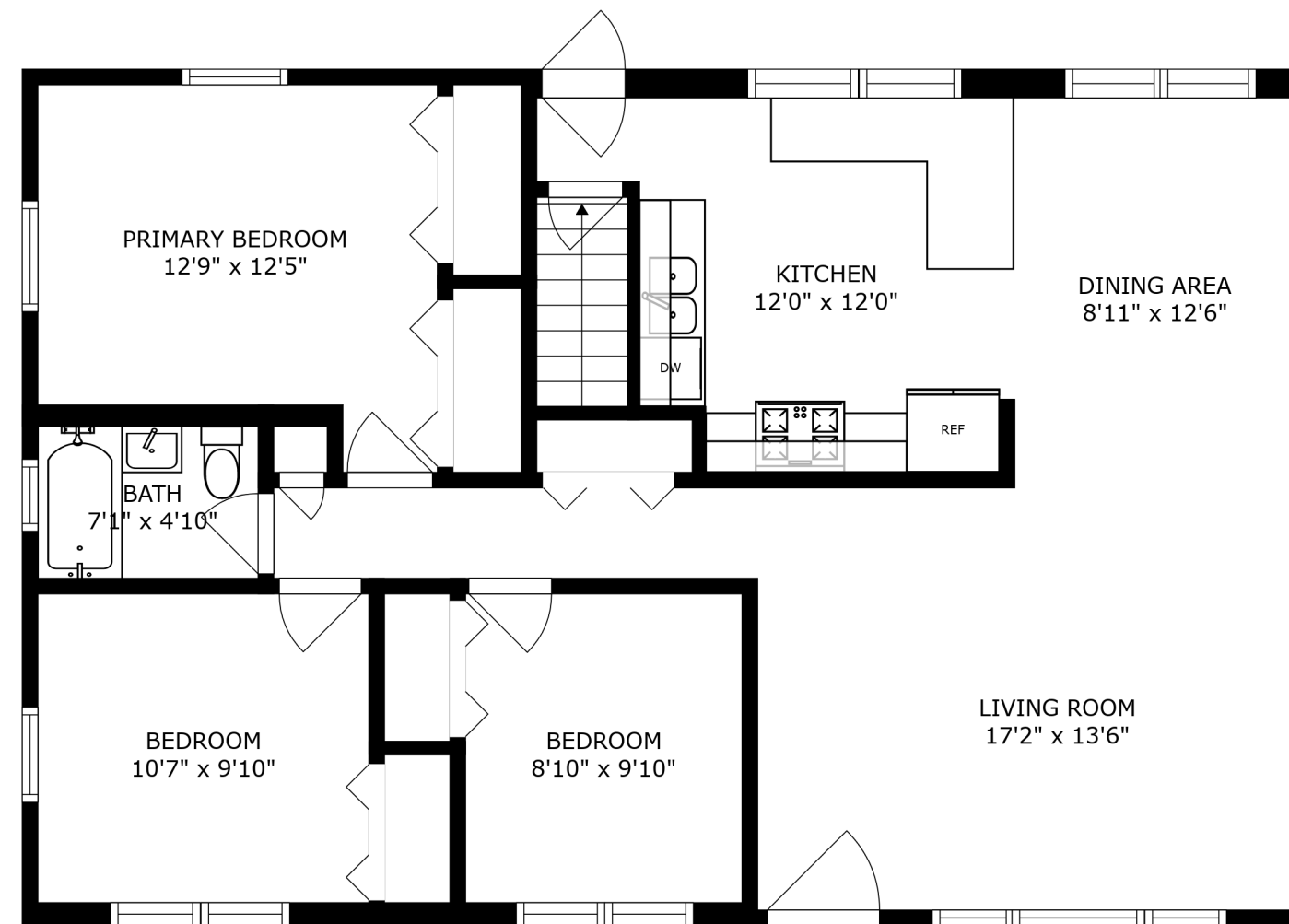
FLOOR 2
