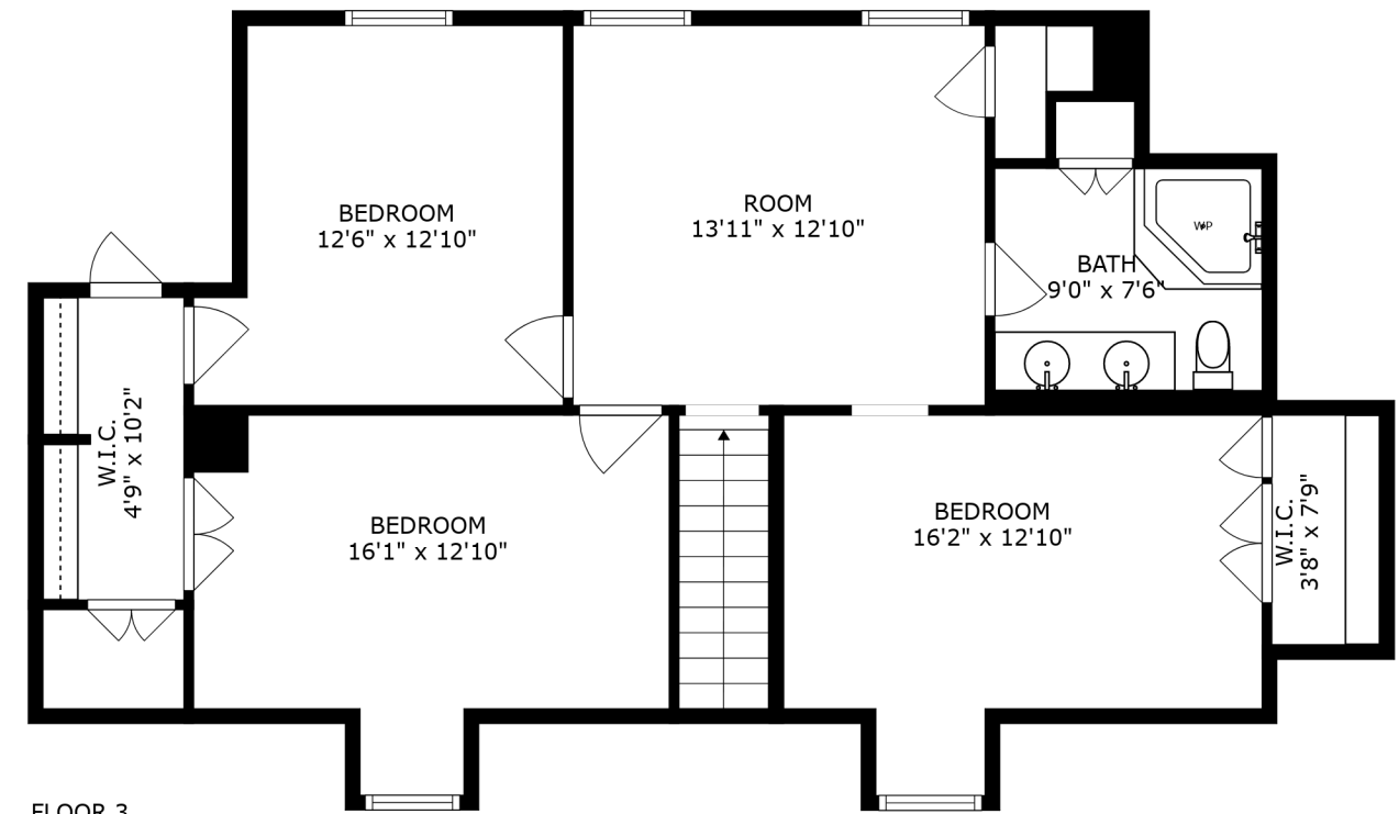
FLOOR 3
