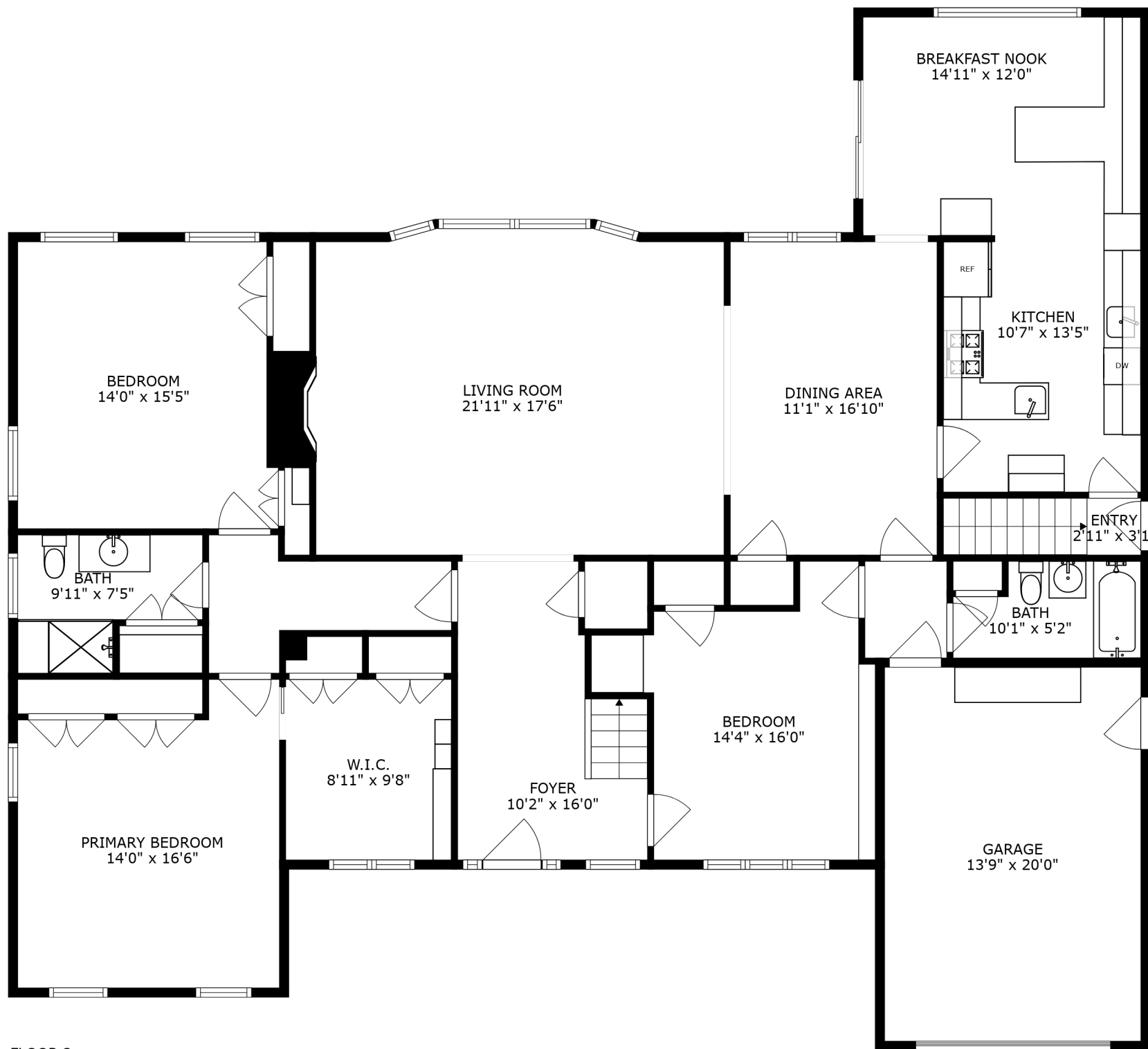
FLOOR 2
