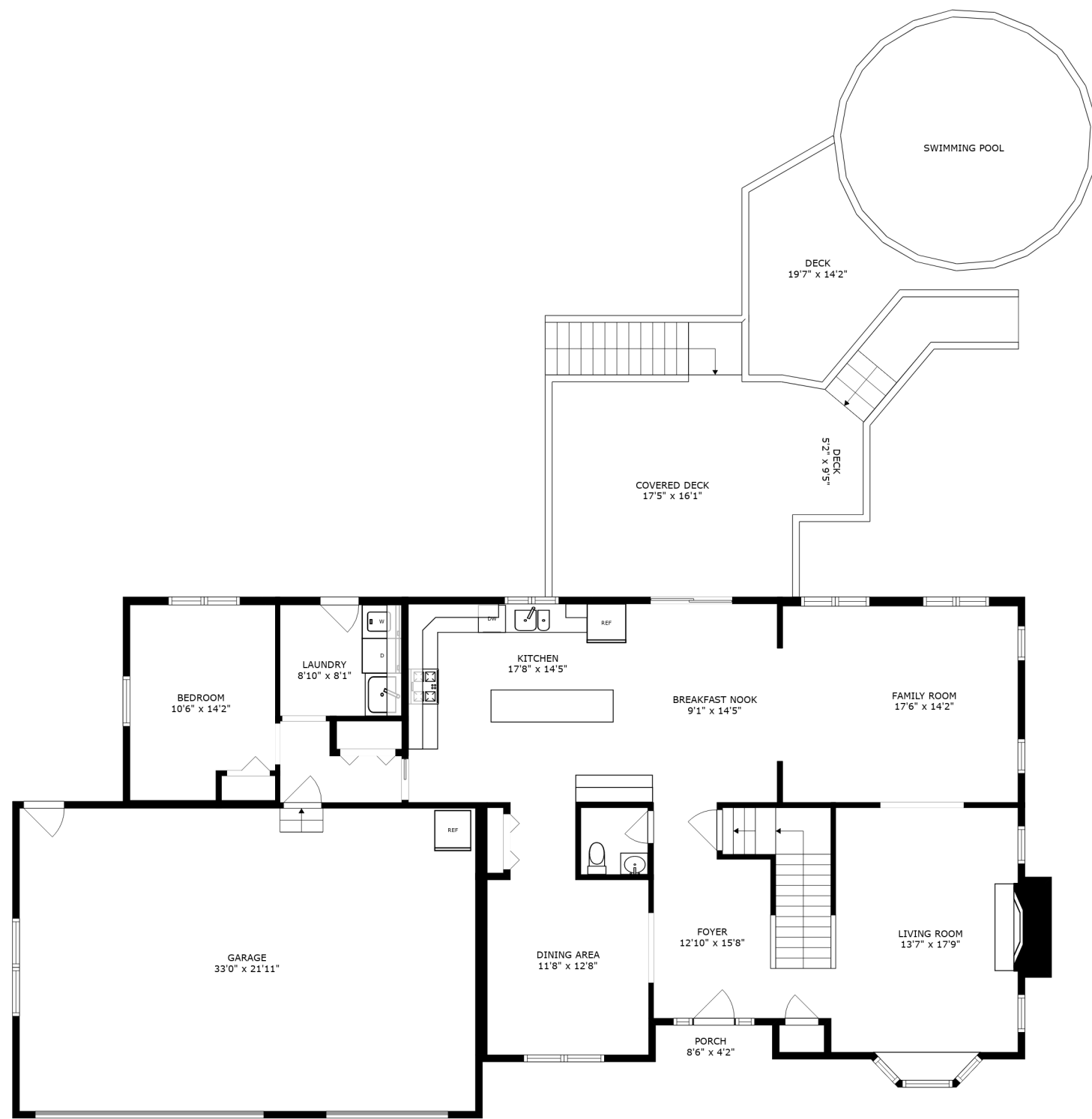
FLOOR 2
