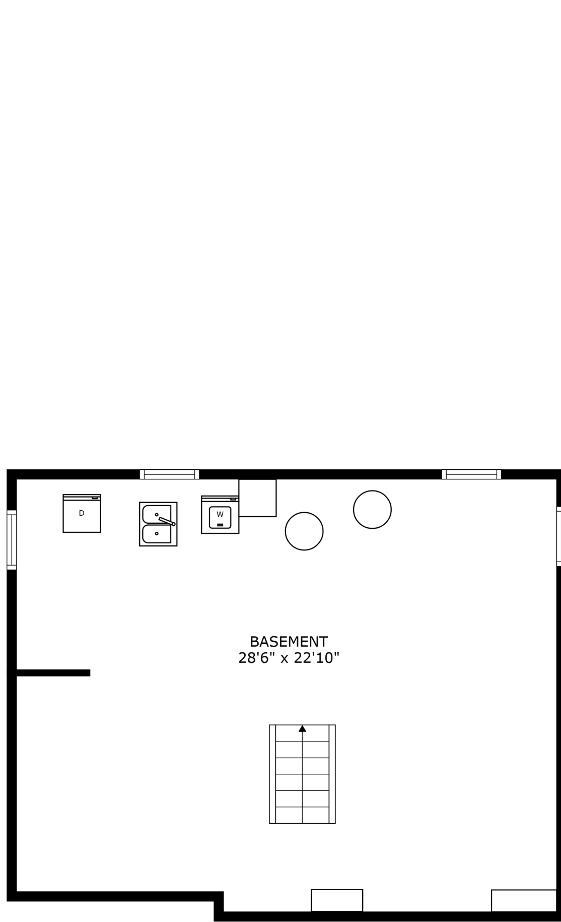
FLOOR 1
