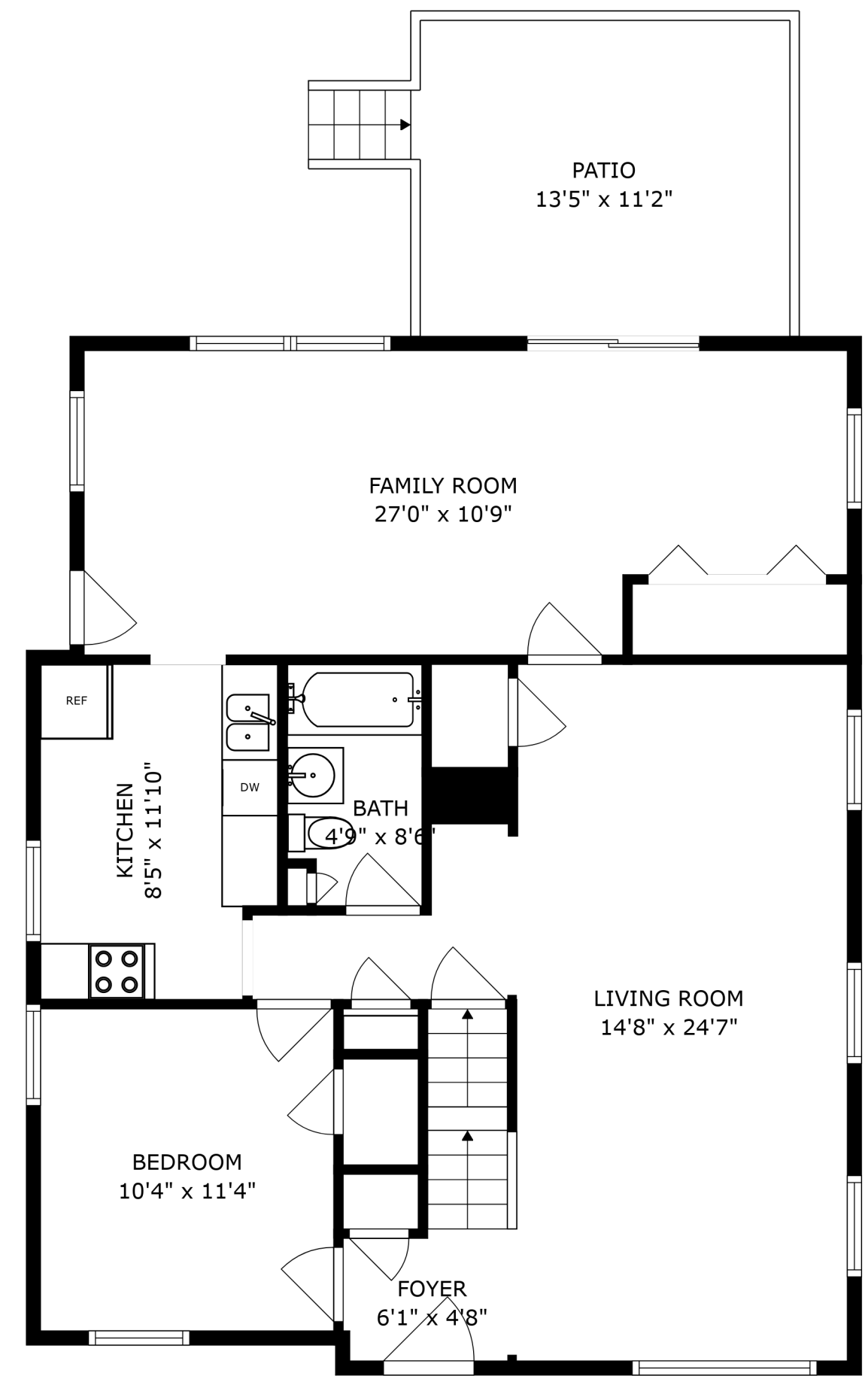
FLOOR 2
