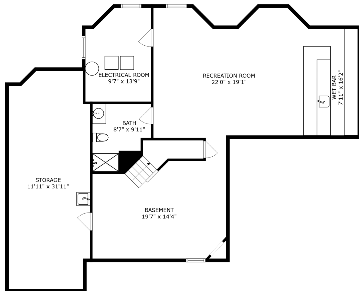
FLOOR 2
