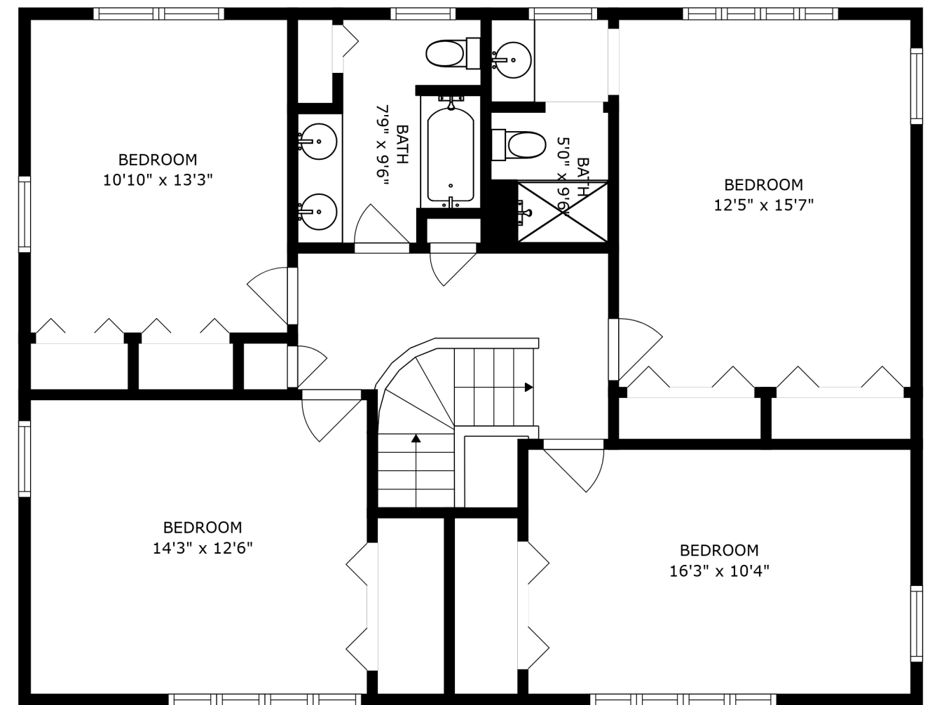
FLOOR 3
