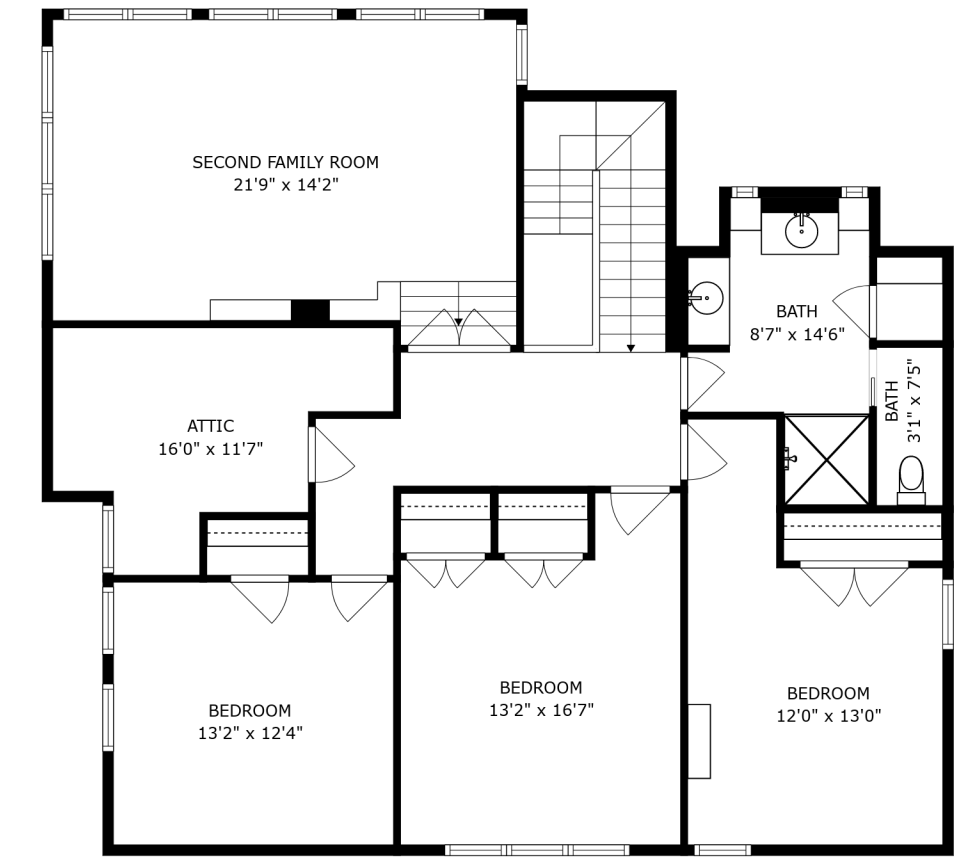
FLOOR 4
