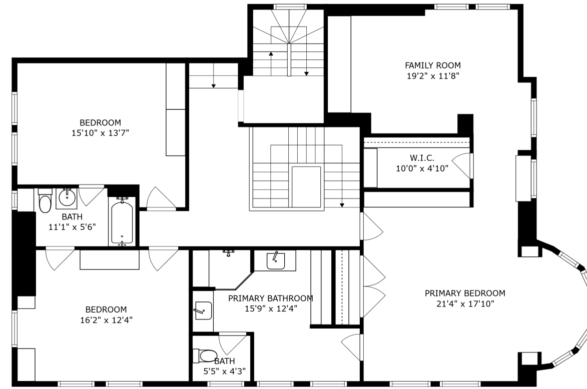
FLOOR 3
