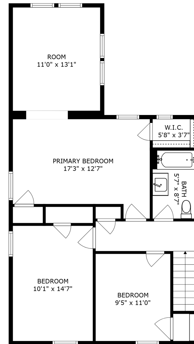
FLOOR 3
