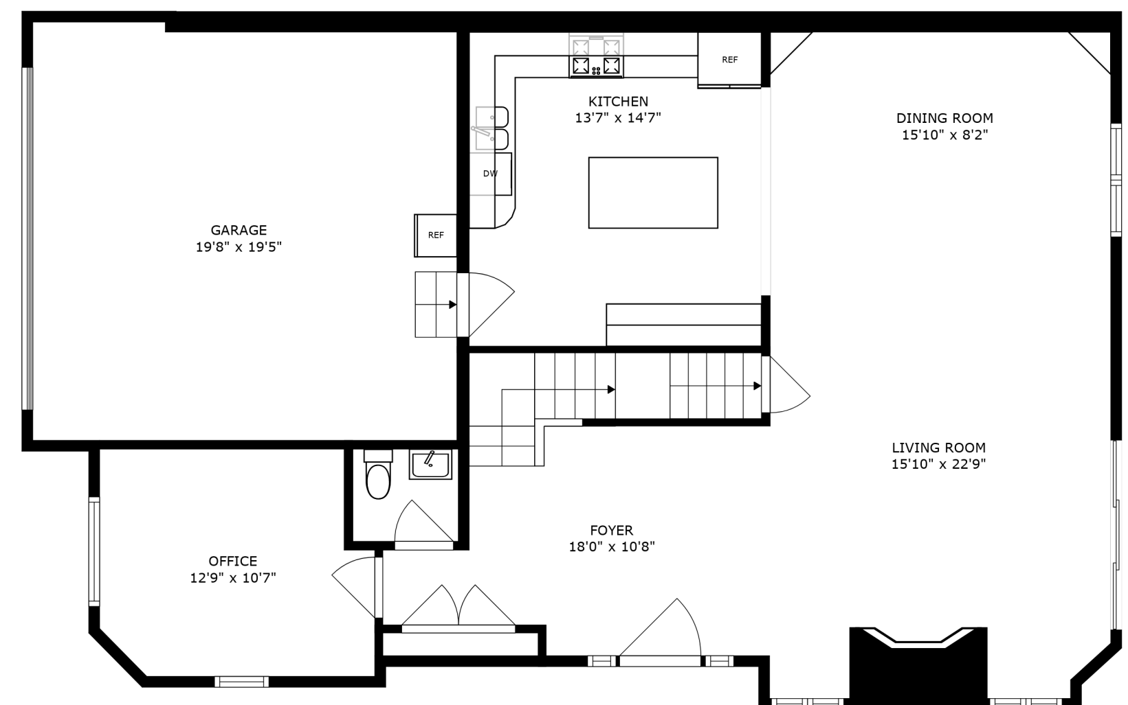
FLOOR 2
