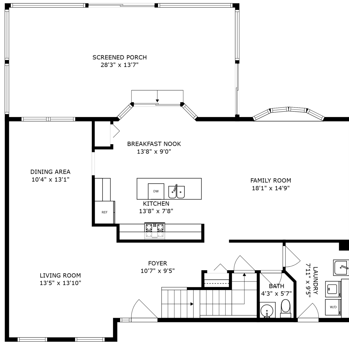
FLOOR 2
