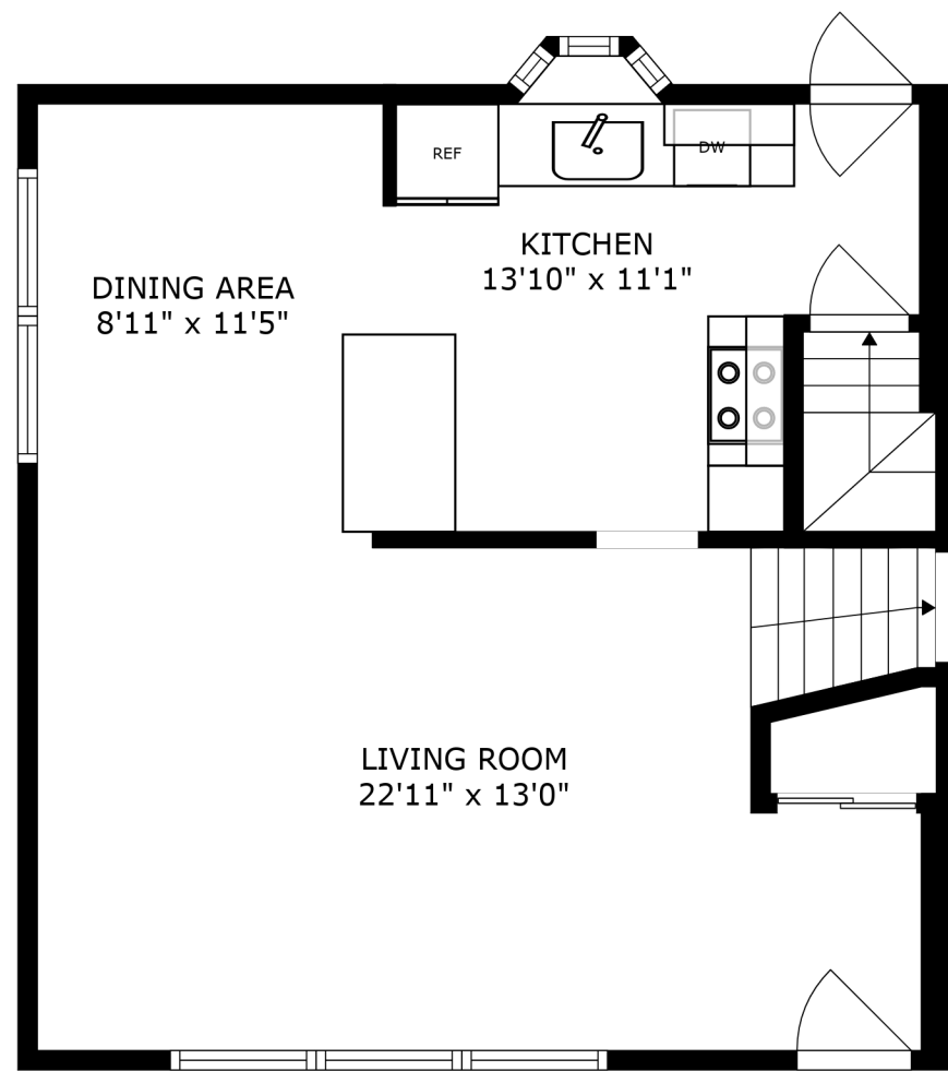
FLOOR 2
