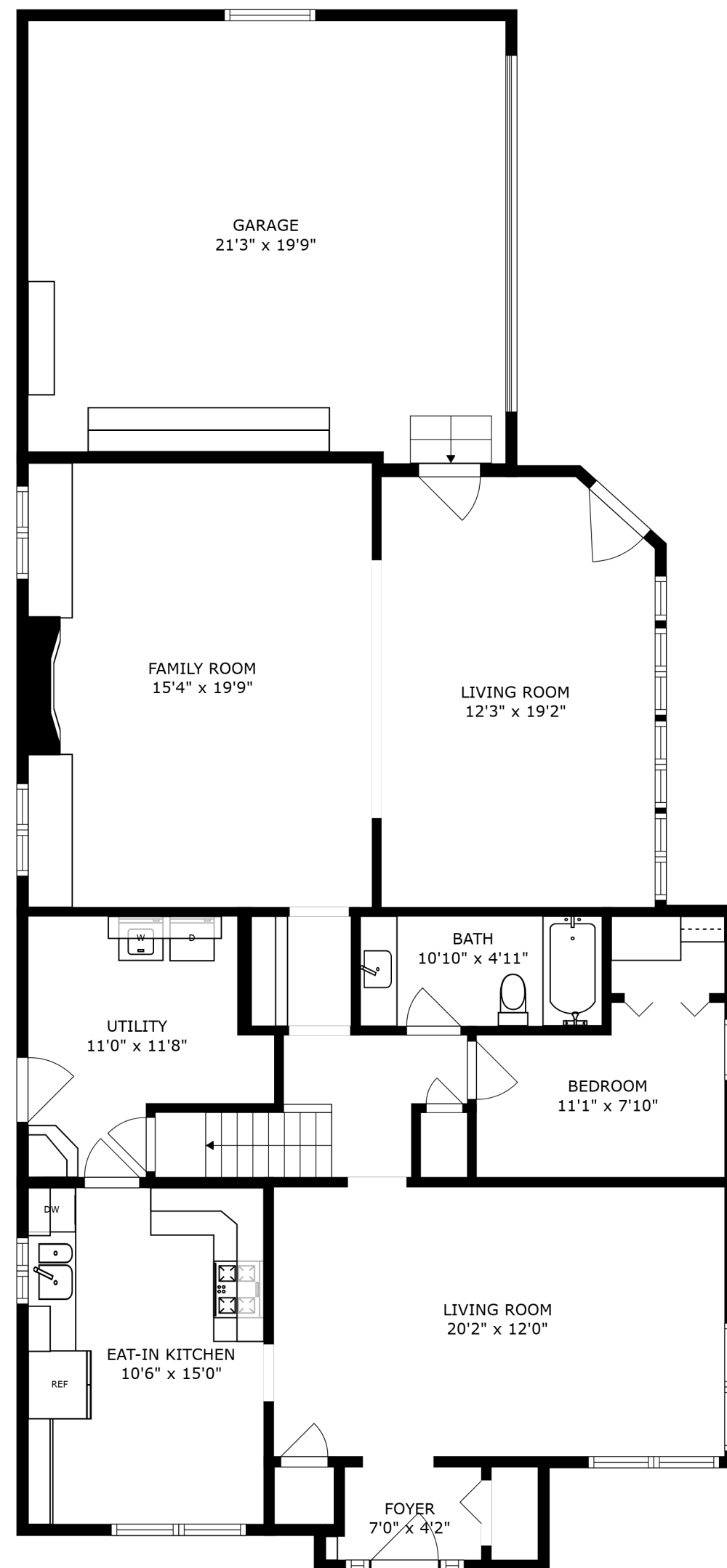
FLOOR 1
