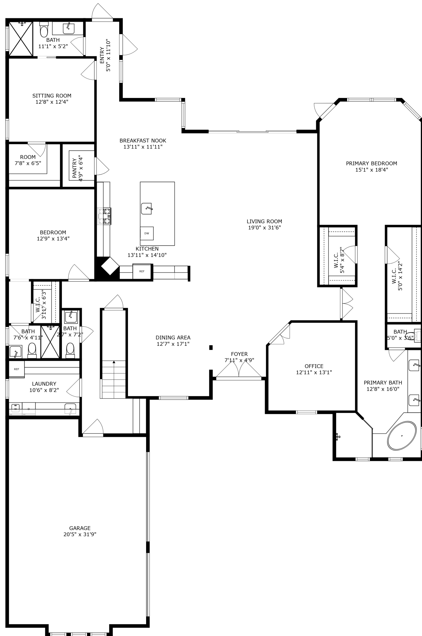
FLOOR 1
