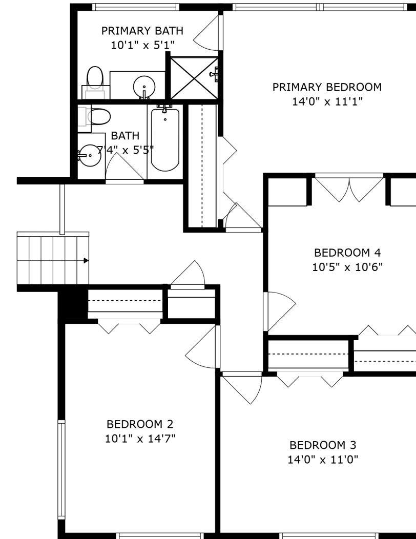
SECOND FLOOR
