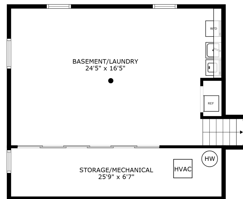
BASEMENT
