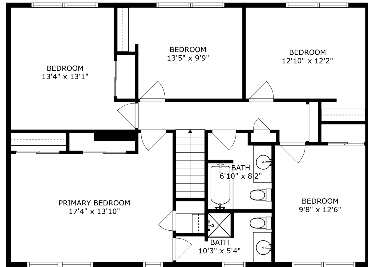
FLOOR 3
